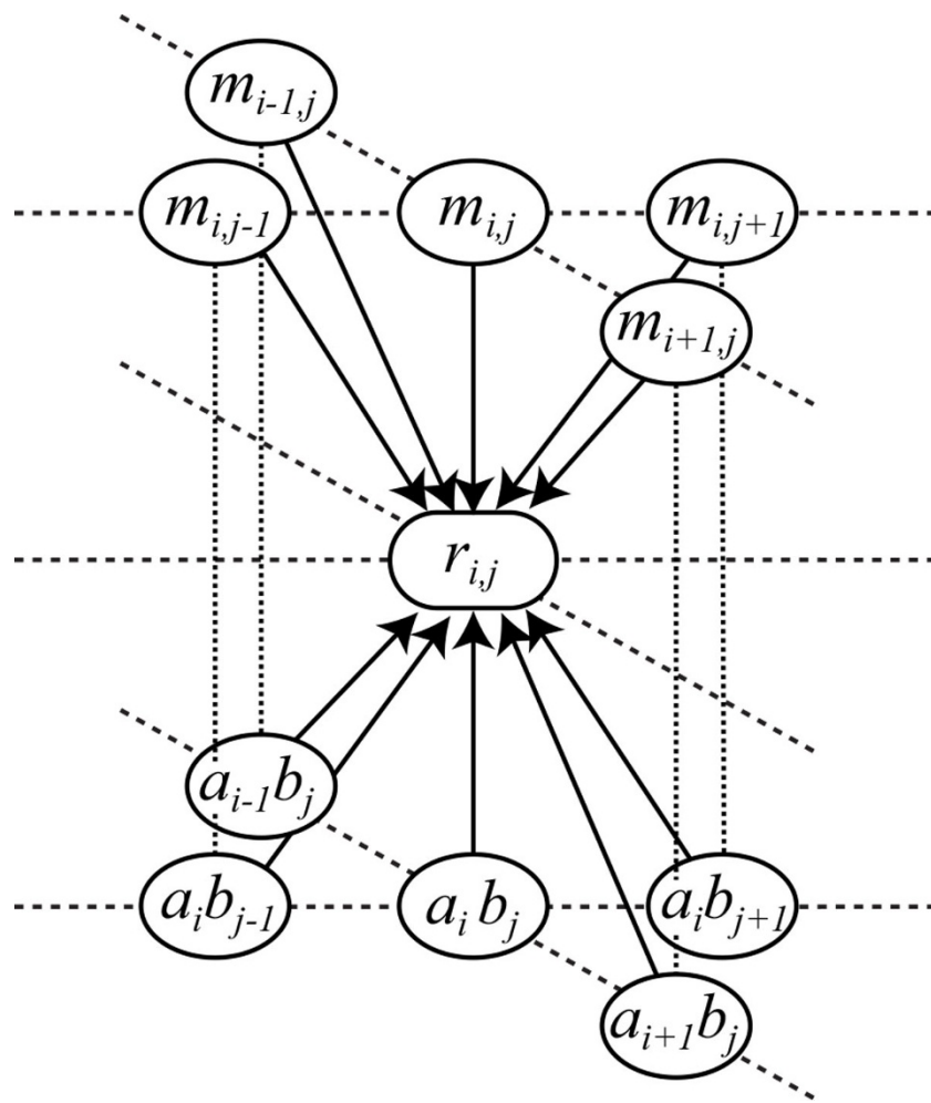
Figure 3 Relationship between the random variable r_{ij} and observations in our CRF model. Relationship between the random variable r_{ij} and the observations of mutual information m_{ij} and the pair (a_i, b_j) of the i -th amino acid in protein sequence A and the j -th base in RNA sequence B , in our CRF model.
