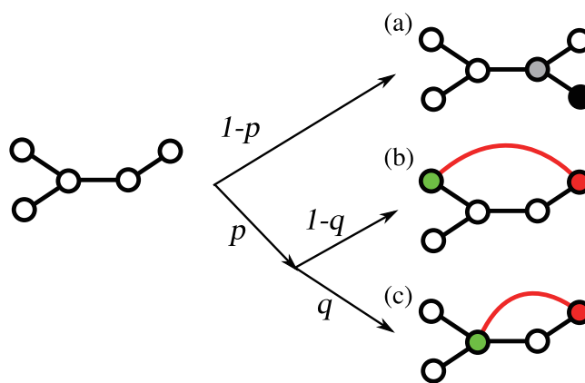
Figure 1 Schematic diagram of the growth mechanisms of the model. (a) Event I. The black and gray nodes are a new node and a randomly selected existing node, respectively. (b) and (c) Event II. The red lines correspond to new edges. The red nodes are randomly selected existing nodes. The green nodes are existing nodes, which are selected by a random walk from each red node. The new edge becomes a short-cut path between the red node and the green node.
