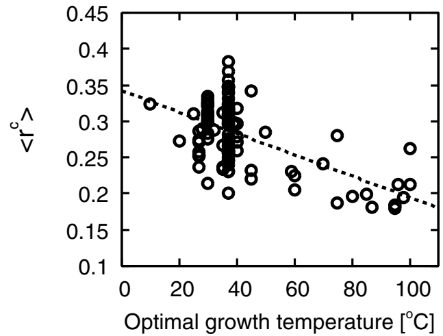
Figure 9 Correlation between the cycle index and temperature. Pearson's correlation r = -0.60 with P < 10^{-11} , Spearman's rank correlation r_s = -0.34 with P < 0.001 .
