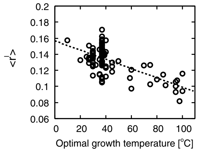
Figure 10 Correlation between the cycle length index and temperature. Pearson's correlation r = -0.63 with P < 10^{-13} , Spearman's rank correlation r_s = -0.33 with P < 0.001 .
