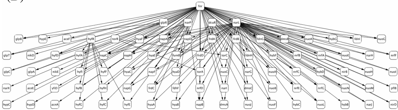
Figure 5 Networks with 5% significance probability in graph consistency search. By corresponding between the regulatory relationships and the gene functions in EcoCyc [44], 29 regulatory networks were reconstructed, and their consistency with the expression profiles measured under anaerobic conditions (accession number GSE1107 in NCBI Gene Expression Omnibus (GEO); http://www.ncbi.nlm.nih.gov/geo/ ) [25] was examined. Among the 29 regulatory networks, two networks showed 5% significance probability: the network related with carbon compounds (EcoCyc ID: C9449_11) (A) and that with anaerobic respiration (EcoCyc ID: C9490_1) (B). The details of the network structures of the 29 regulatory networks are shown in the additional file 6: the 29 network structures analyzed in the present study.
