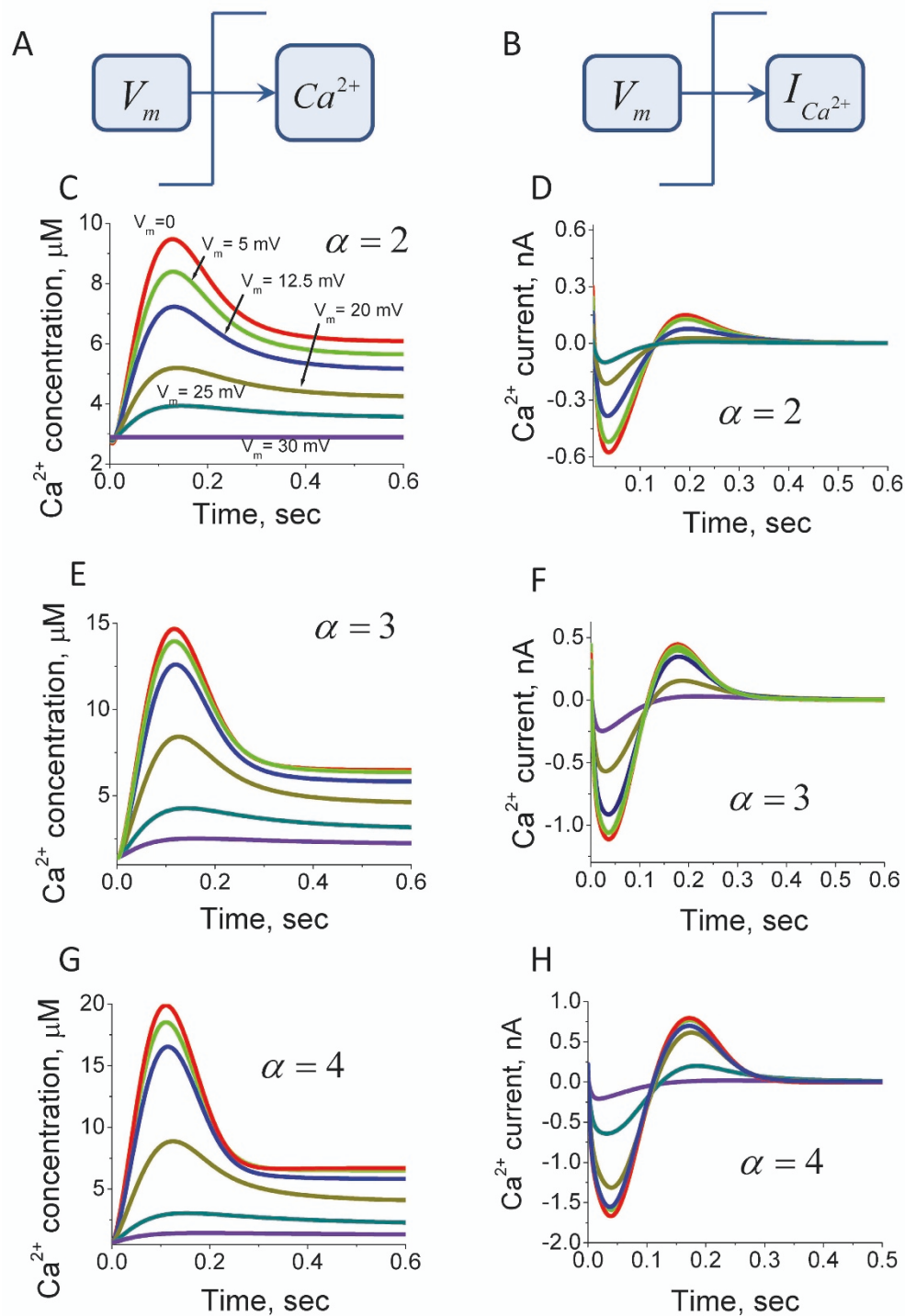
Figure 3 Systems model predictions for intraciliary Ca^{2+} concentration and current responses to the transmembrane potential shift. The intraciliary Ca^{2+} concentrations (A) and Ca^{2+} currents (B) are calculated according to the model with direct Ca^{2+} -mediated ciliary Ca^{2+} channels inhibition in response to variable degree of transmembrane potential shift. The responses are colour coded according to the degree of applied transmembrane potential shift. The violet and red coloured lines represent dynamic responses obtained after the smallest and the largest depolarising shift of membrane potential, respectively. The non dimensional membrane potential values following voltage shift from initial \psi_0 = -1.2 are shown in (C) and remain the same throughout the figure. The calculations suggest that ciliary membrane depolarisation induces an intraciliary Ca^{2+} spike over a wide physiological range of depolarising conditions (C, E and G), whereas the current generates a biphasic response (D, F and H). The calculations were carried out for three different levels of parameter \alpha , which reflects the steepness of the Ca^{2+} channels conductivity dependence on membrane potential.
