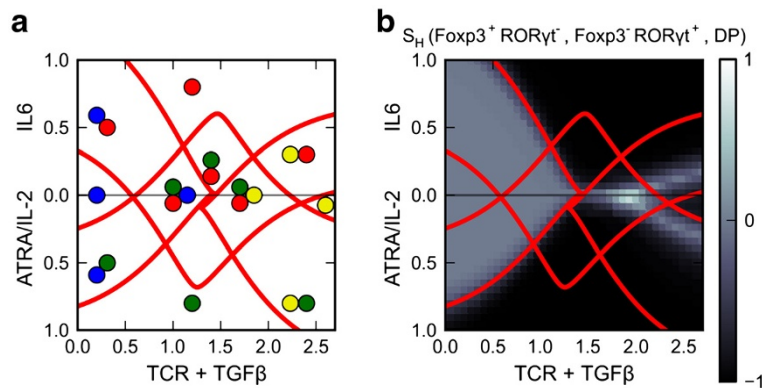
Figure 8 Analyses of Prototype Model 3 (heterogeneous differentiation of iT_{Reg} and T_H17 cells). a. Bidirectional two-parameter bifurcation diagram with respect to primary signal TCR + TGF- \beta and polarizing signals ATRA/IL2 and IL-6. Adjoined circles: multistability. Blue circle: naive phenotype. Green circle: Foxp3 single-positive phenotype. Red circle: ROR \gamma t single-positive phenotype. Yellow: DP phenotype. b. Simulation results of induced differentiation. The heterogeneity scores with respect to Foxp3 single-positive phenotype, ROR \gamma t single-positive phenotype and DP phenotype are shown.
