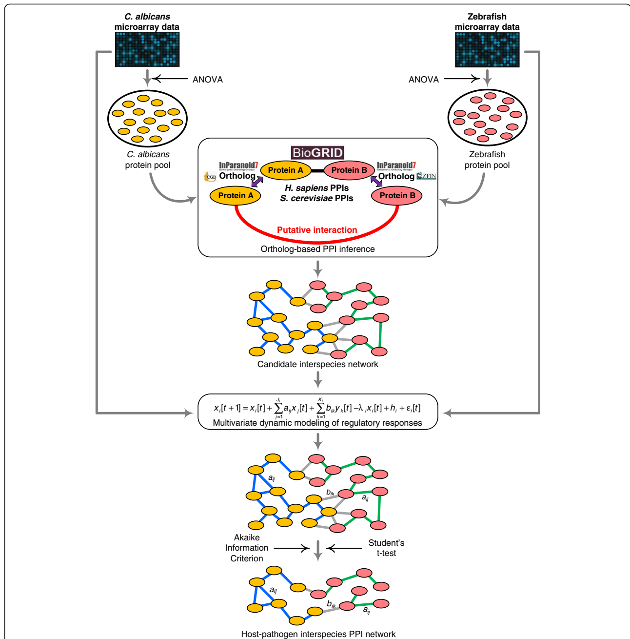
Figure 1 Schematic overview of the interspecies protein-protein interaction network construction framework. Protein-protein interaction (PPI) data from the BioGRID database, ortholog information from CGD, ZFIN, InParanoid, and simultaneous time-course microarray data for both C. albicans and zebrafish during C. albicans -zebrafish interactions were used for interspecies PPI network construction. On the basis of the PPI data for S. cerevisiae and H. sapiens and the ortholog information among these related species, putative interspecies and intracellular PPIs were inferred, which constitute the candidate interspecies network. Then, using multivariate dynamic modeling of regulatory responses and simultaneously quantified microarray data, the regulatory abilities were identified, and the significant interactions determined. In this manner, the candidate interspecies network and the refined host-pathogen interspecies PPI network, yellow and pink nodes indicate C. albicans and zebrafish proteins, where blue, green, and grey edges denote C. albicans intracellular interactions, zebrafish intracellular interactions, and interspecies interactions, respectively.
